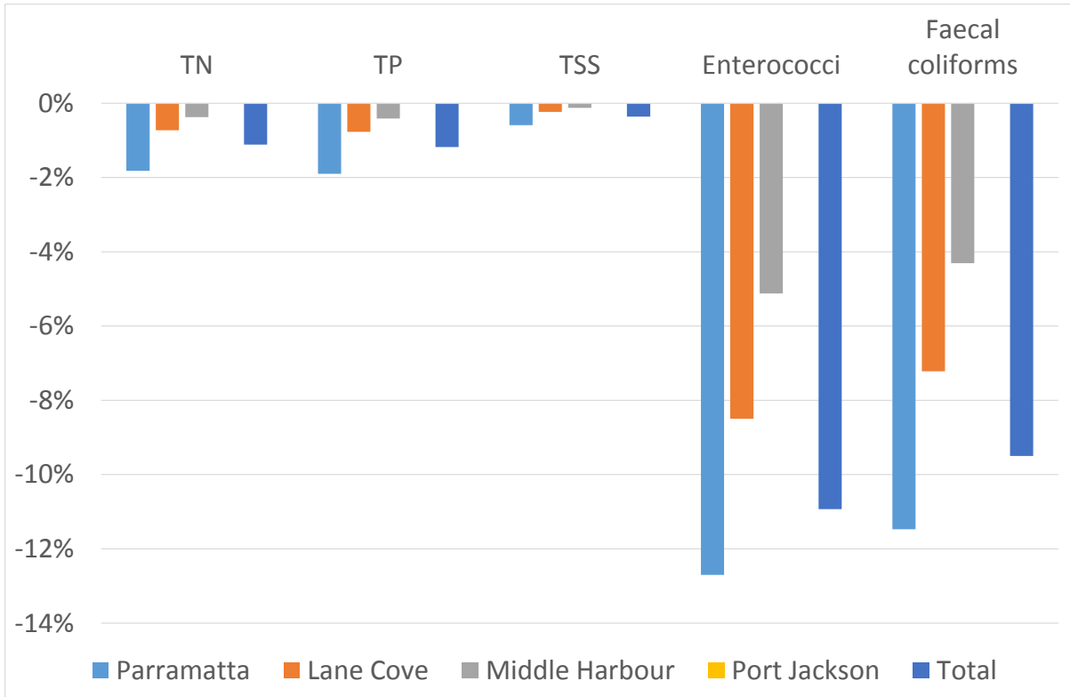
FIGURE 20. IMPACT OF LIMITING SEWER OVERFLOWS TO 40 EVENTS IN 10 YEARS ON POLLUTANT LOADS
