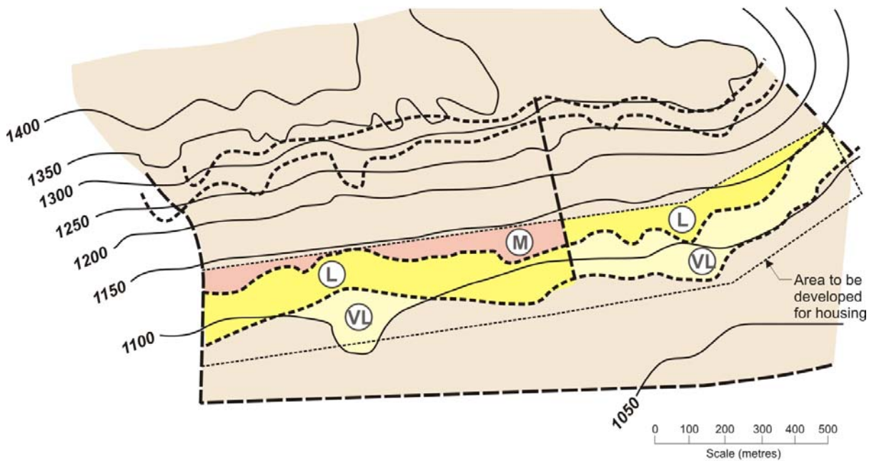
Figure 2C Rockfall Risk
